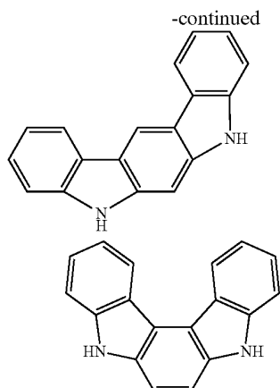
Indolocarbazole (crosslinked with a nitrogen atom)
