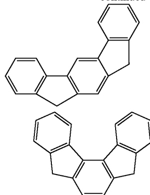
Indeno[1,2-b]fluorene (crosslinked with a carbon atom)
