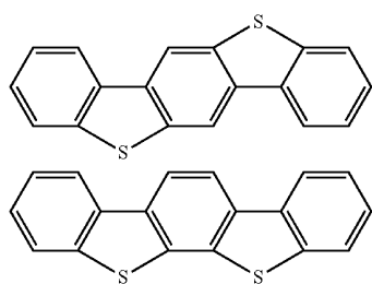
Benzofuranodibenzofuran (crosslinked with an oxygen atom)
