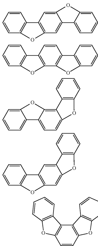
Benzofuranodibenzofuran (crosslinked with an oxygen atom)
